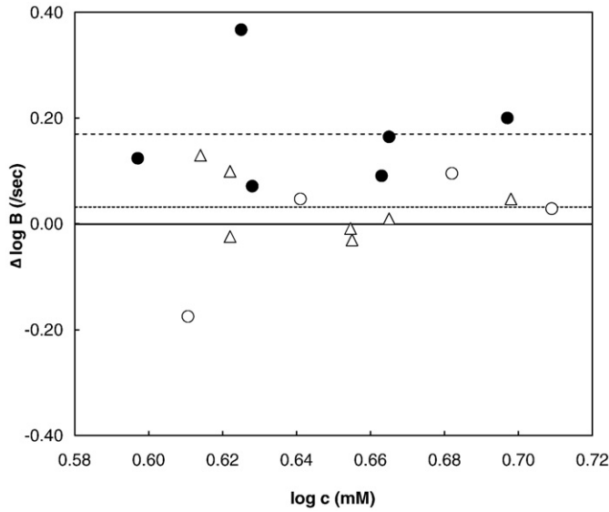
Fig. 2. Log of exponential growth rate B after subtracting a second order polynomial fit to HbS without cdb3, plotted as a function of log of initial HbS concentration. B is dominated by the square root of the heterogeneous nucleation rate, and changes only slightly due to the homogeneous nucleation rate. The polynomial used was \log B = -27 + 68 \log c - 39 (\log c)^2 . Filled circles show Hb with the strong binding variant (cdb3+), while open circles show the weak binding variant (cdb3-). Open triangles show HbS in the same buffer without any cdb3, to which the polynomial was fit. The solid line is the fit to HbS+, the long dashed line is the average of the deviations of HbS with cdb3+ while the dotted line is the average of the deviations of HbS with cdb3- from the polynomial. \log B is clearly greater for the filled symbols.
